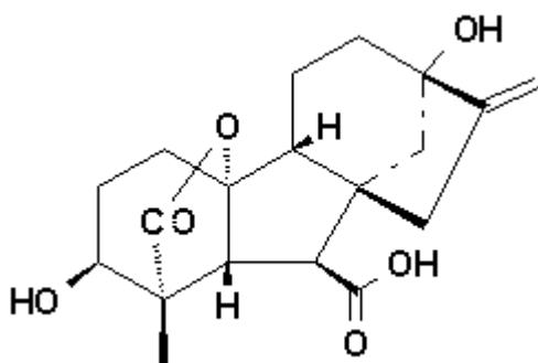
(Fig.- Structure of Gibberellin)
